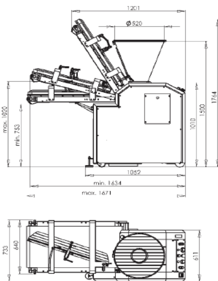
Rounding device 90 cm with belt 2120 x 490 mm
