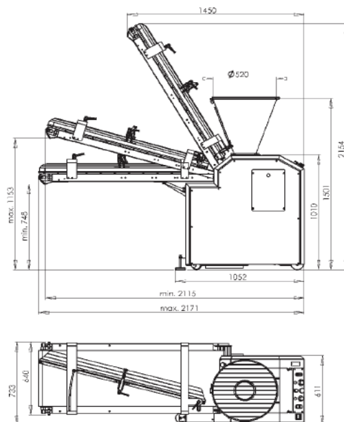
Rounding device 140 cm with belt 3120 x 490 mm
