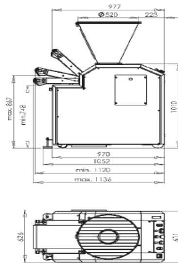
Short belt 1050 x 277 mm or 1312 x 277 mm
